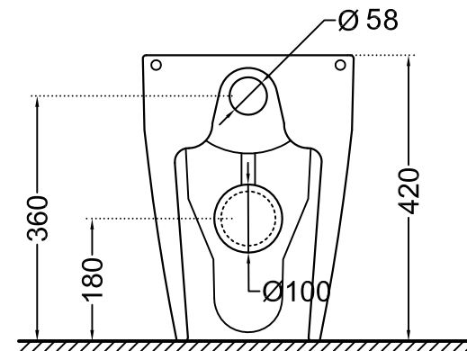
BACK VIEW
